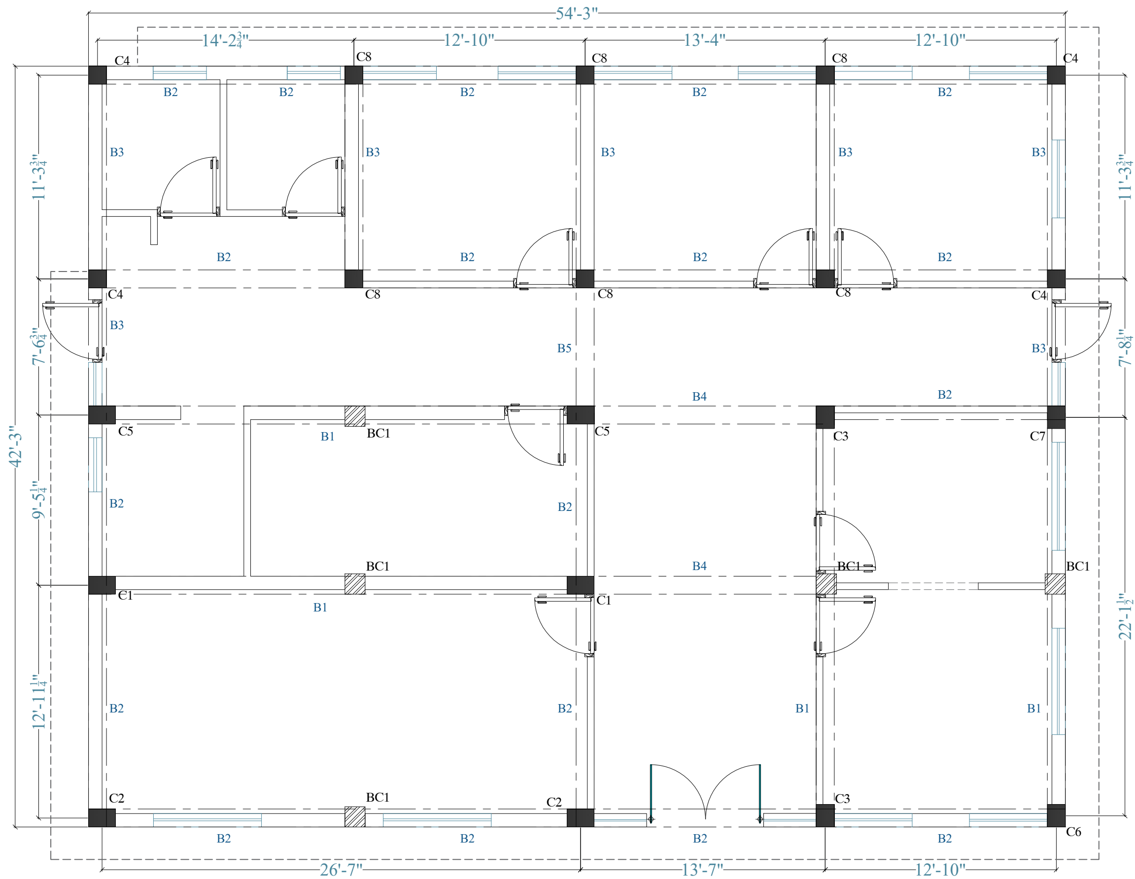
BEAM LAYOUT
